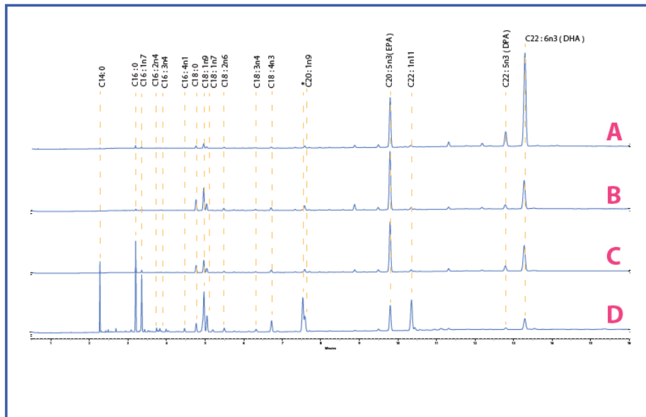
Figure 2. Chromatographic separation of FAME compounds found present in the three omega 3 supplements and the standard fish oil obtained with the Sapiens-FAMEWAX 20m x 0.18mm x 0.18µm capillary column. Trace A, B, C correspond to Samples A, B, C respectively and trace D corresponds to PUFA n° 1 standard.
